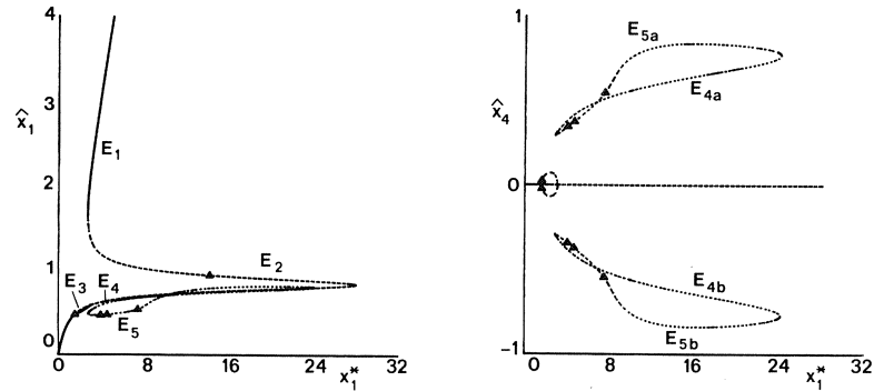
FIGURE 5.2. Stationary solutions of the 10-component model. Shown are the \hat{x}_1 - and \hat{x}_4 -component as a function of x_1^* for b = 1.6, \beta = 1.25, C = 0.1, \gamma = 1 and x_4^* = 0 . A solid line denotes that the solution is stable whereas a dashed line refers to an unstable solution. Hopf bifurcation points are indicated by a triangle.
