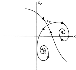
FIGURE 2.5. Sketch of the phase flow of the three component-model, projected onto the x_1 - x_2 plane in case there are three equilibria. Initial conditions are chosen in a plane x_3 = \text{constant} .
