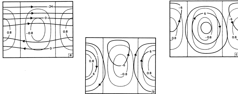
FIGURE 5.6. As figure 5.3, but for the equilibria EQ_1, EQ_2 and EQ_3 defined in (5.2).
