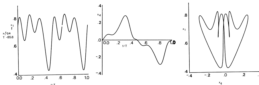
FIGURE 3.8. Visualization of some periodic orbits occurring for b=2 , case I. Shown are x_1(t/T) , x_4(t/T) and a projection of the orbits onto the x_1-x_4 plane. Here t is time and T the period.
