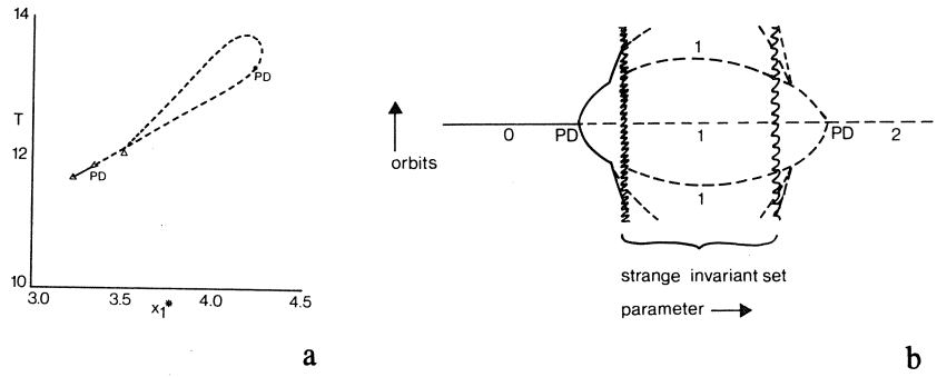
FIGURE 3.13. a. As figure 3.7, but for the cases III and IV. b. Bifurcation scheme in the region between the period-doubling bifurcations of figure 3.13a. The straight line denotes the principal periodic orbit. The number of Floquet multipliers with absolute values larger than 1 (which measures the degree of instability of the periodic orbits) is also indicated.
