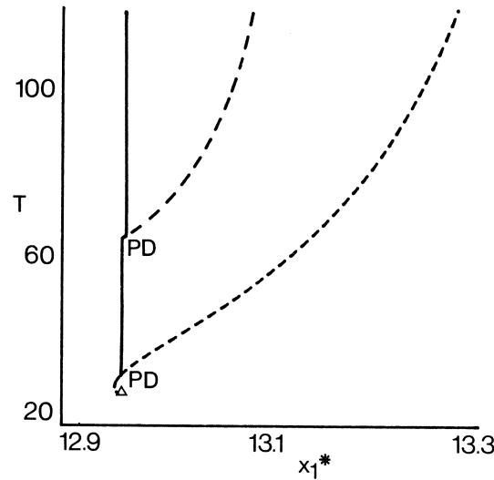
FIGURE 3.5 Period T of the periodic orbits as a functions of x_1^* for b=1.6 . Stability properties are denoted by a solid curve (stable) or a dashed curve (unstable). A Hopf bifurcation is indicated by a triangle, a period-doubling bifurcation by PD .
