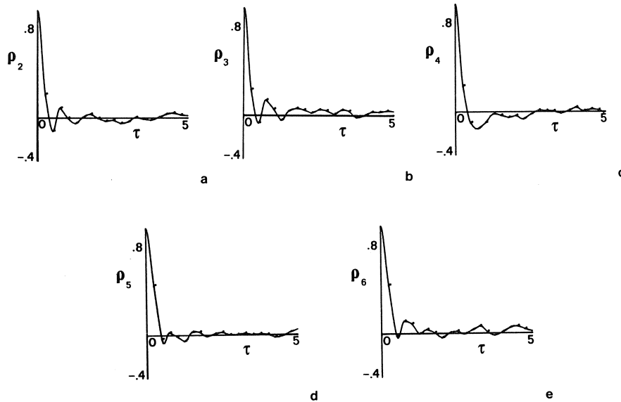
FIGURE 5.15. Autocorrelation functions \rho_i(\tau) of the forcing terms F_i(t) ( i=2,3,4,5,6 ) acting on the six-component model.
