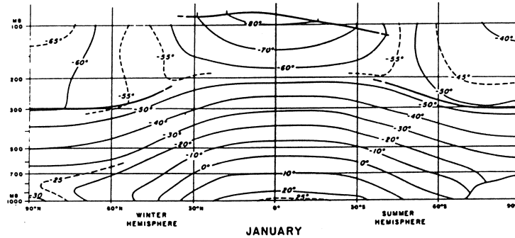
FIGURE 1.1 Mean temperature distribution, averaged around latitude circles, for January. Heavier lines show approximate mean tropopauses. From PALMÉN and NEWTON (1969).
