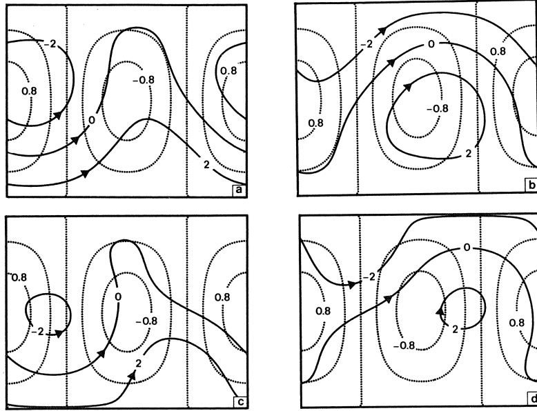
FIGURE 5.3. Nondimensional streamfunction contours (solid lines) for the equilibria E_{4a}(a), E_{4b}(b), E_{5a}(c) and E_{5b}(d) defined in (5.1). A difference \Delta\psi=1 corresponds to a zonal transport of about 1.1 \cdot 10^6 m^2 s^{-1} . The dashed lines represent contours of topography ( 10^3 m ).
