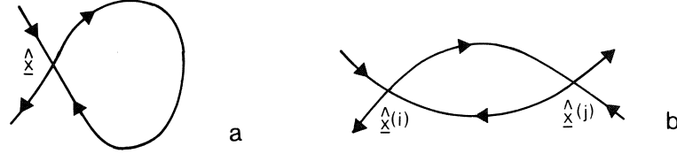
FIGURE D1. Visualization of homoclinic (a) and heteroclinic connections (b).
